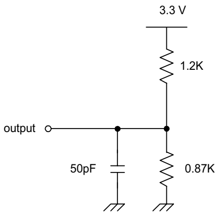
AC TEST LOAD (A)
