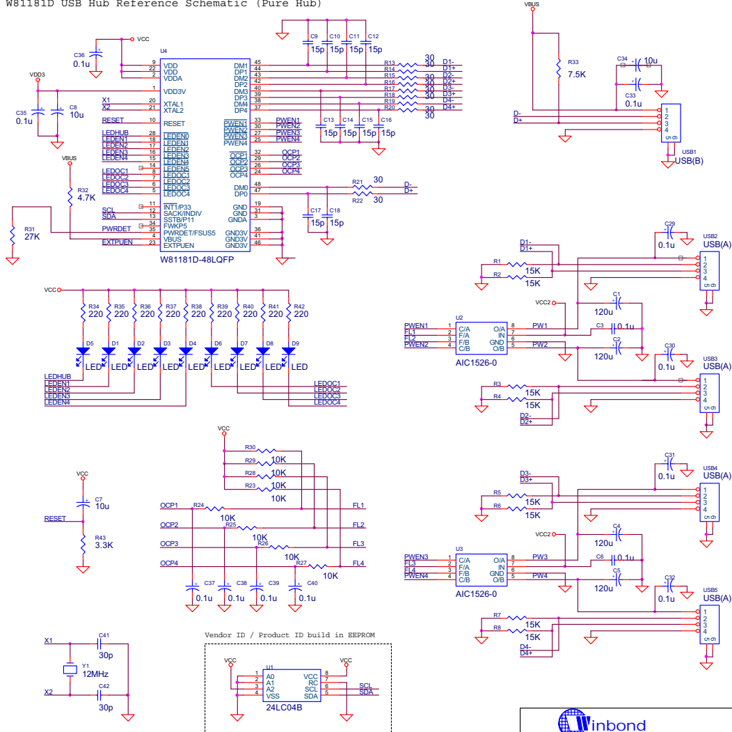
W81181D USB Hub Reference Schematic (Pure Hub)
